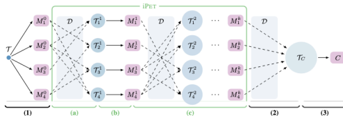
Figure 2: Schematic representation of PET (1-3) and iPET (a-c). (1) The initial training set is used to finetune an ensemble of PLMs . (a) For each model, a random subset of other models generates a new training set by labeling examples from \mathcal{D} . (b) A new set of PET models is trained using the larger, model-specific datasets. (c) The previous two steps are repeated k times, each time increasing the size of the generated training sets by a factor of d . (2) The final set of models is used to create a soft-labeled dataset \mathcal{T}_C . (3) A classifier C is trained on this dataset.
